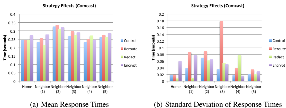
Figure 4.6: Non-Hierarchical Results from Comcast
